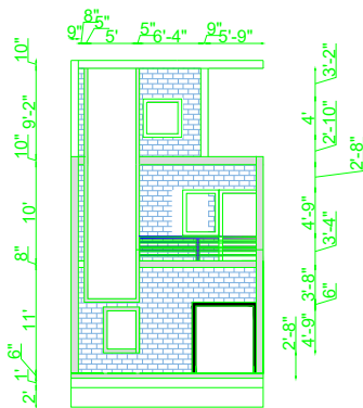
FRONT SECTION
